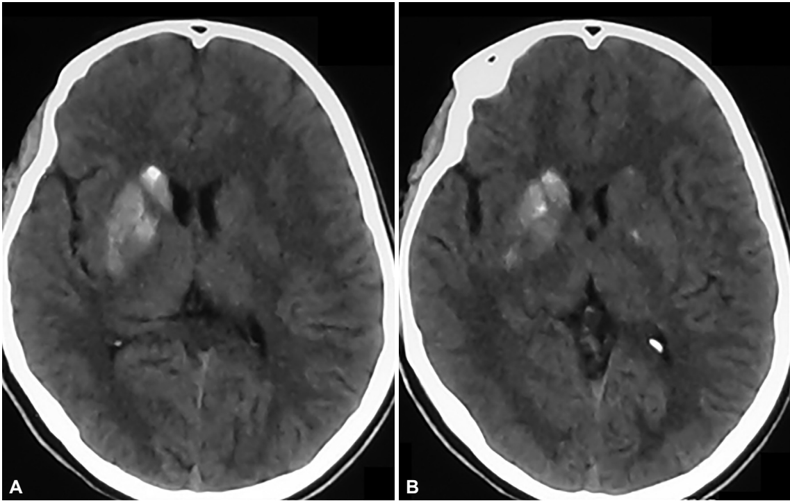
Supplementary Figure 1. Brain CT in our case, showing diffuse hyperdensity of the right caudate and lentiform nuclei (A, B) and subtle hyperdensity involving the left caudate and lentiform nuclei (B).
