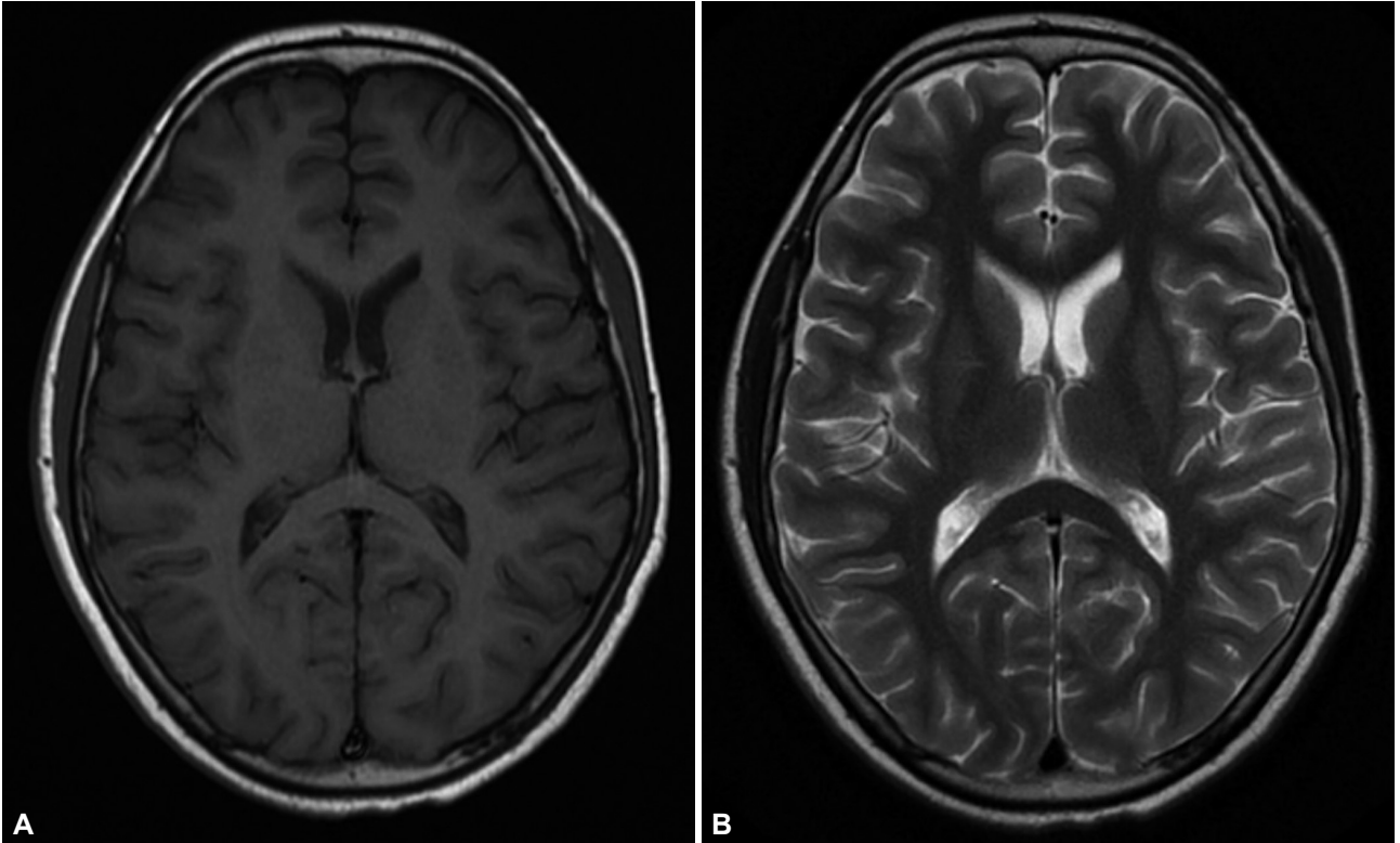
Supplementary Figure 1. Brain MRI showing normal axial T1 (A) and T2 (B) sequences.
